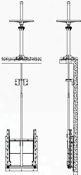
MODEL S11-P
