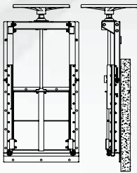
MODEL S22-Y
