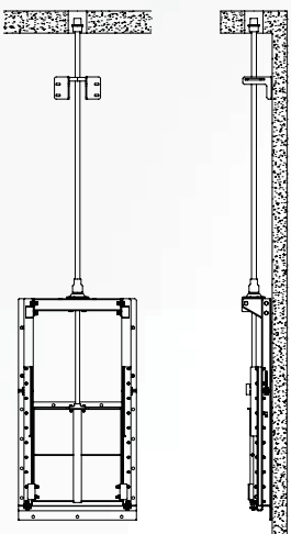
MODEL S22-F
